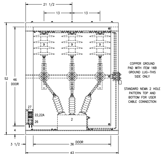
Typical Surge Equipment Drawing
